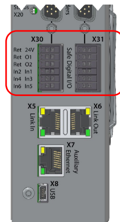
Figure 23: Digital I/O connector (X30+X31)
