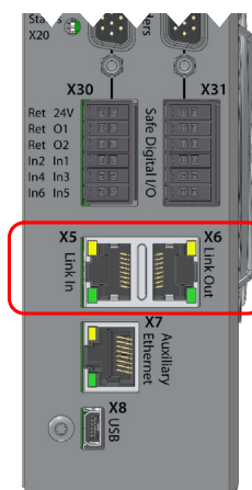
Figure 13: Link jacks (X5, X6)
