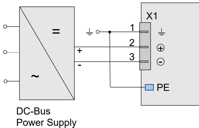
Figure 5: DC-Bus connection
