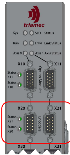
Figure 19: Encoder jack (X20,X21)
