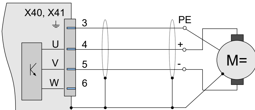
Figure 29: DC-motor connection
