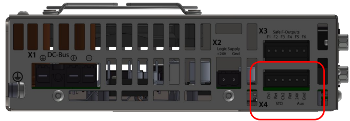
Figure 12: STO connector (X4)
