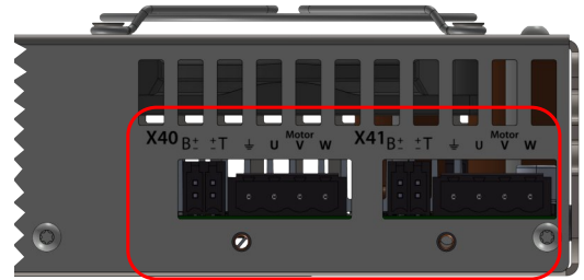
Figure 31: Motor temperature and Brake connector
