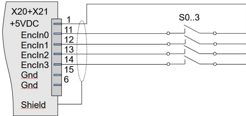
Figure 23: TTL input connection
