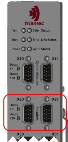
Figure 17: Encoder jack (X20,X21)
