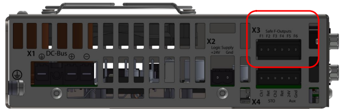
Figure 10: Safe Function Outputs connector (X3)
