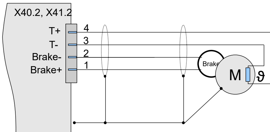
Figure 32: Motor temperature and brake connection
