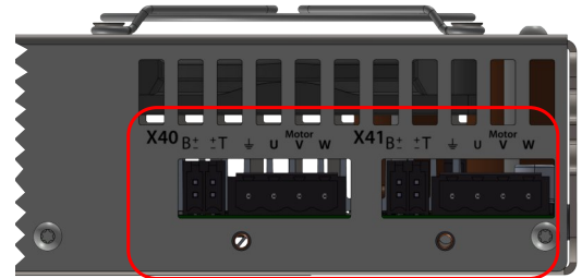
Figure 27: Motor connectors
