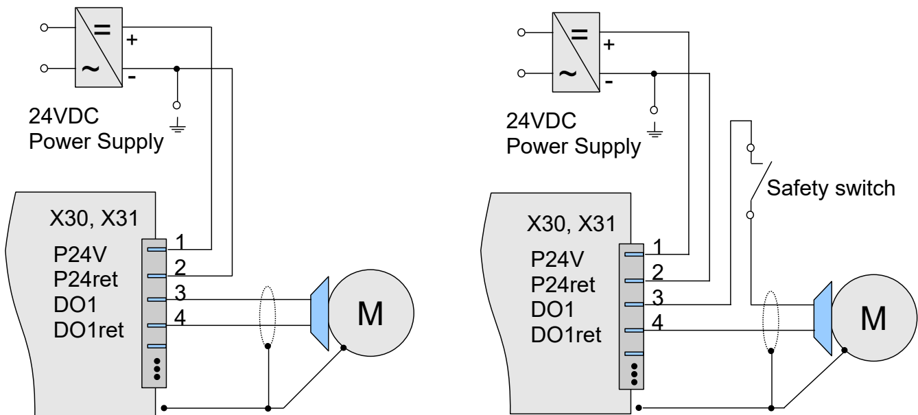
Figure 26: Typical motor brake connection without external safety switch (left), with external safety switch (right)
