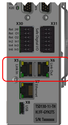
Figure 14: Link jacks (X5, X6)
