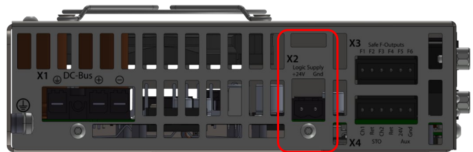
Figure 8: 24V Logic supply connector (X2)
