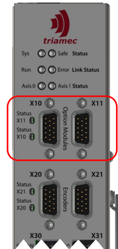
Figure 15: Option module jacks (X10,X11)
