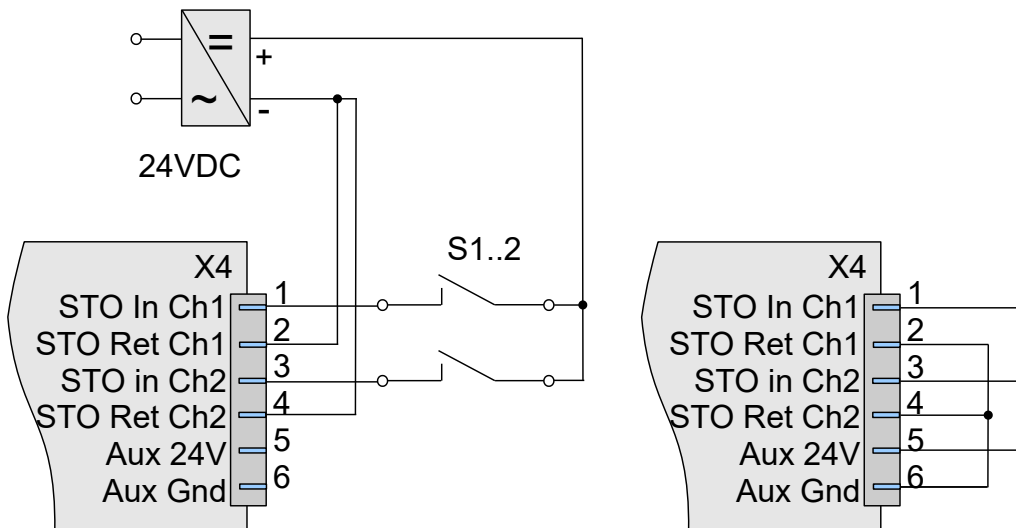
Figure 13: Wiring of the STO used (left) and not used (right)
