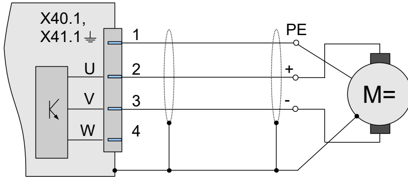
Figure 30: DC-motor connection
