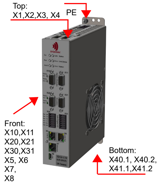
Figure 5: Overview of the connectors
