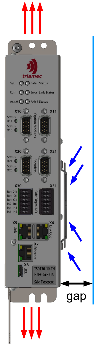
Figure 3: Mounting and cooling
