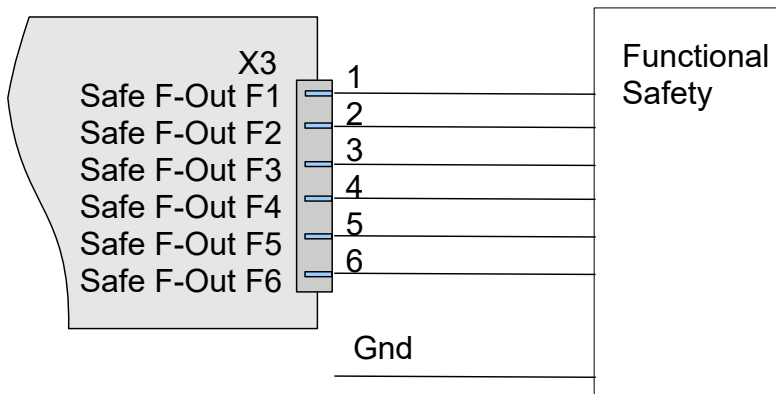
Figure 11: Wiring of the State Outputs
