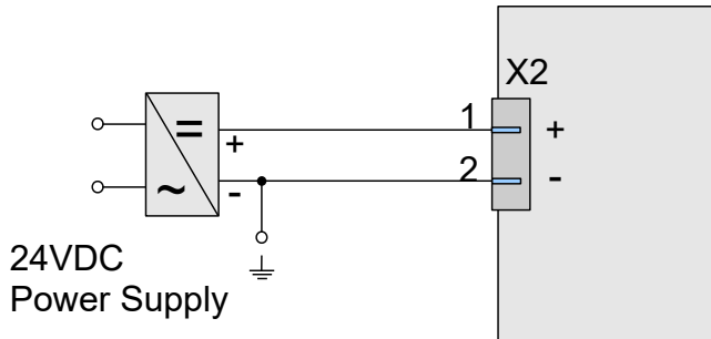
Figure 9: 24VDC logic power supply connection
