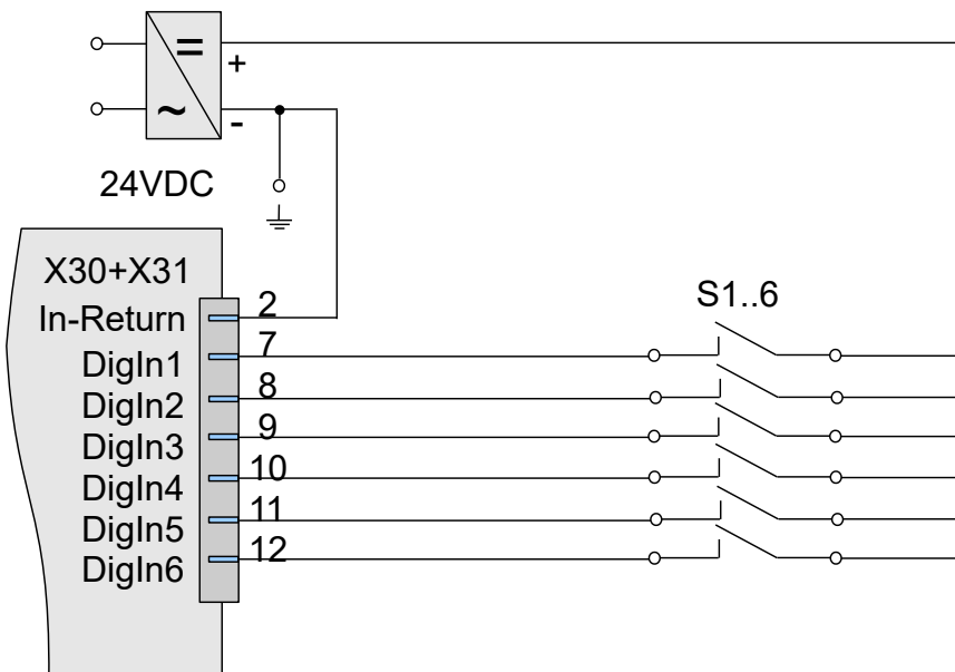
Figure 25: Digital input connection
