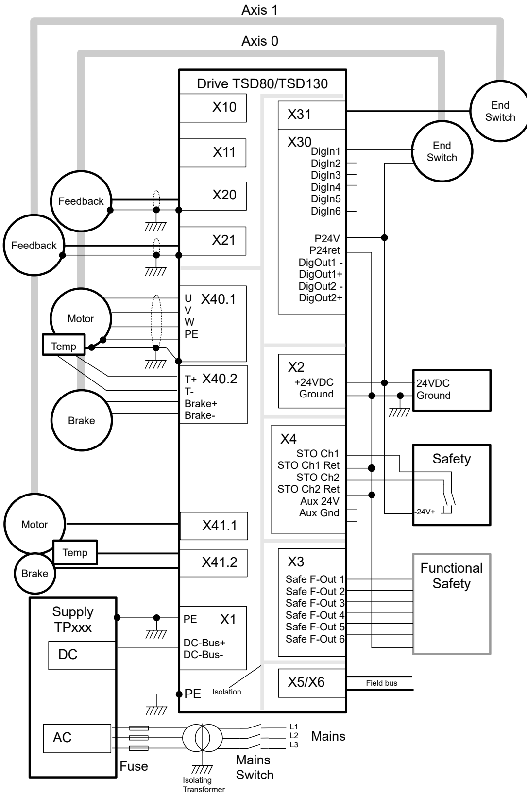
Figure 4: Connection diagram TSD80/TSD130
