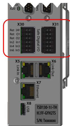
Figure 24: Digital I/O connector (X30+X31)
