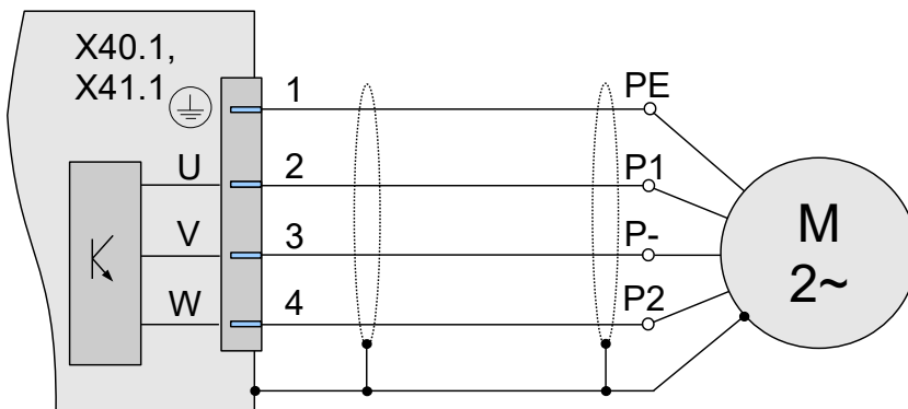
Figure 29: 2-phase motor connection
