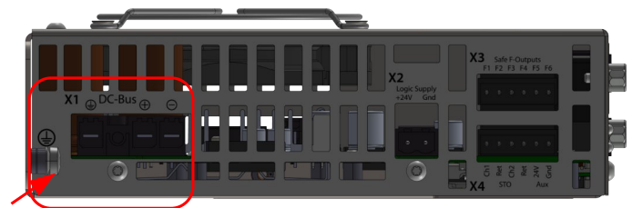
Figure 7: DC-Bus connector (X1)
