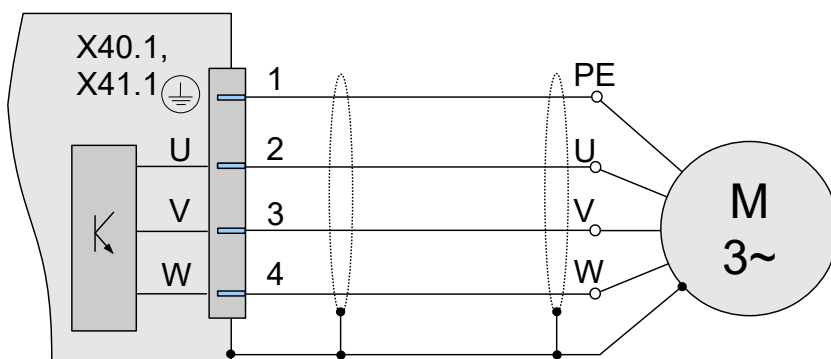
Figure 28: 3-phase motor connection
