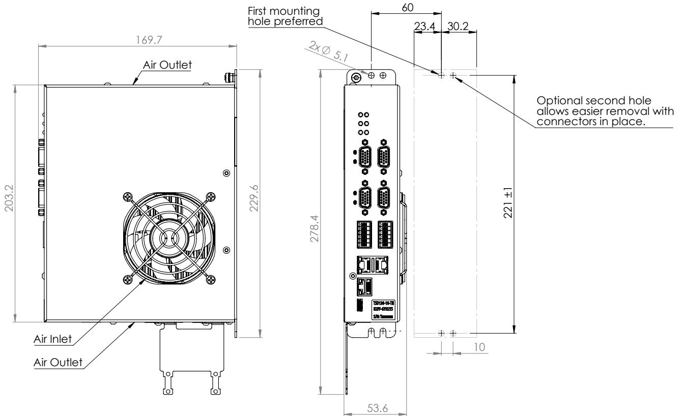
Figure 2: Mechanical Drawing
