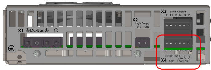
Figure 11: STO connector (X4)
