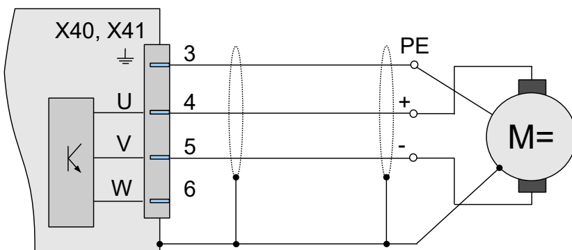
Figure 29: DC-motor connection
