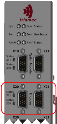
Figure 22: Encoder jack (X20,X21)
