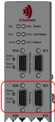
Figure 20: Encoder jack (X20,X21)
