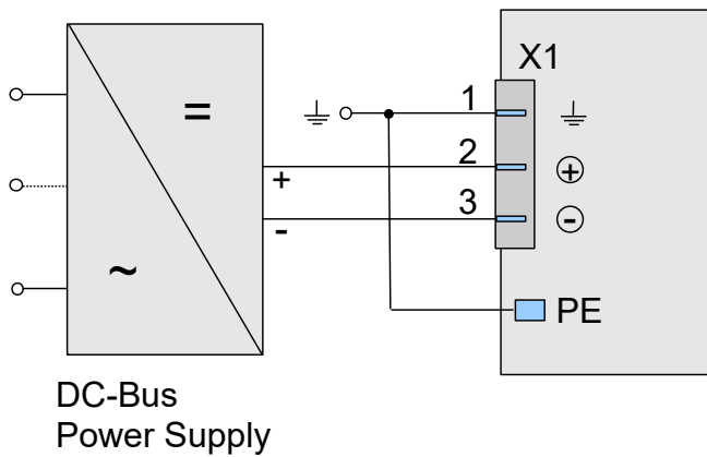
Figure 6: DC-Bus connection
