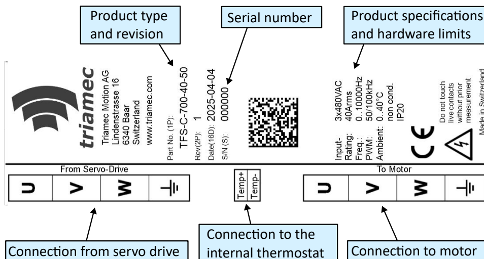
Figure 3: Label of the TFS-C-700-40-50 as an example for all labels of the Triamec Motion AG filter series.
